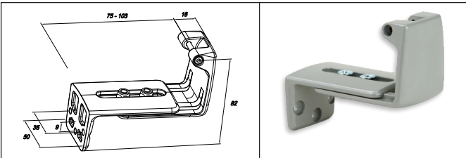
Aluminium adjustable “Z” bracket for bottom hinged window GREY part No. 41709Z BLACK part No. 41710A WHITE part No. 41711B
